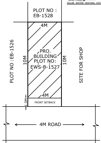
SITE PLAN
