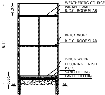
SECTION ON XX
