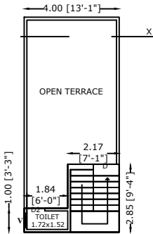
2. SECOND FLOOR PLAN
