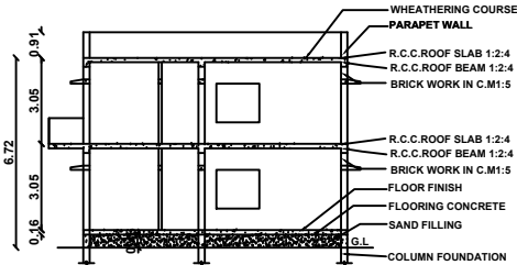
SECTION ON G.G
