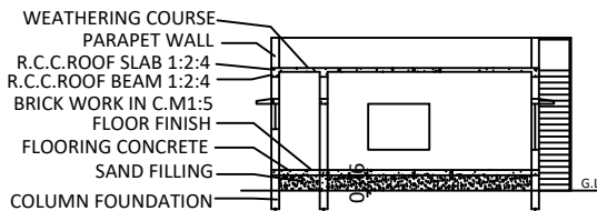
SECTION- SS
