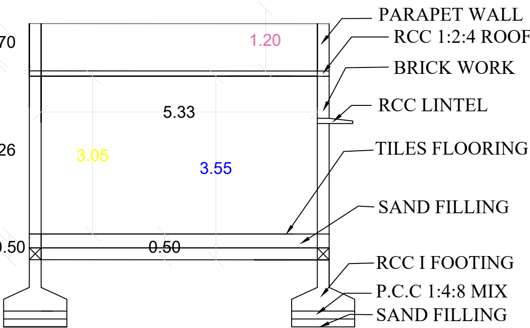
TYPICAL SECTION ON AB PLAN - 1 & PLAN - 2
