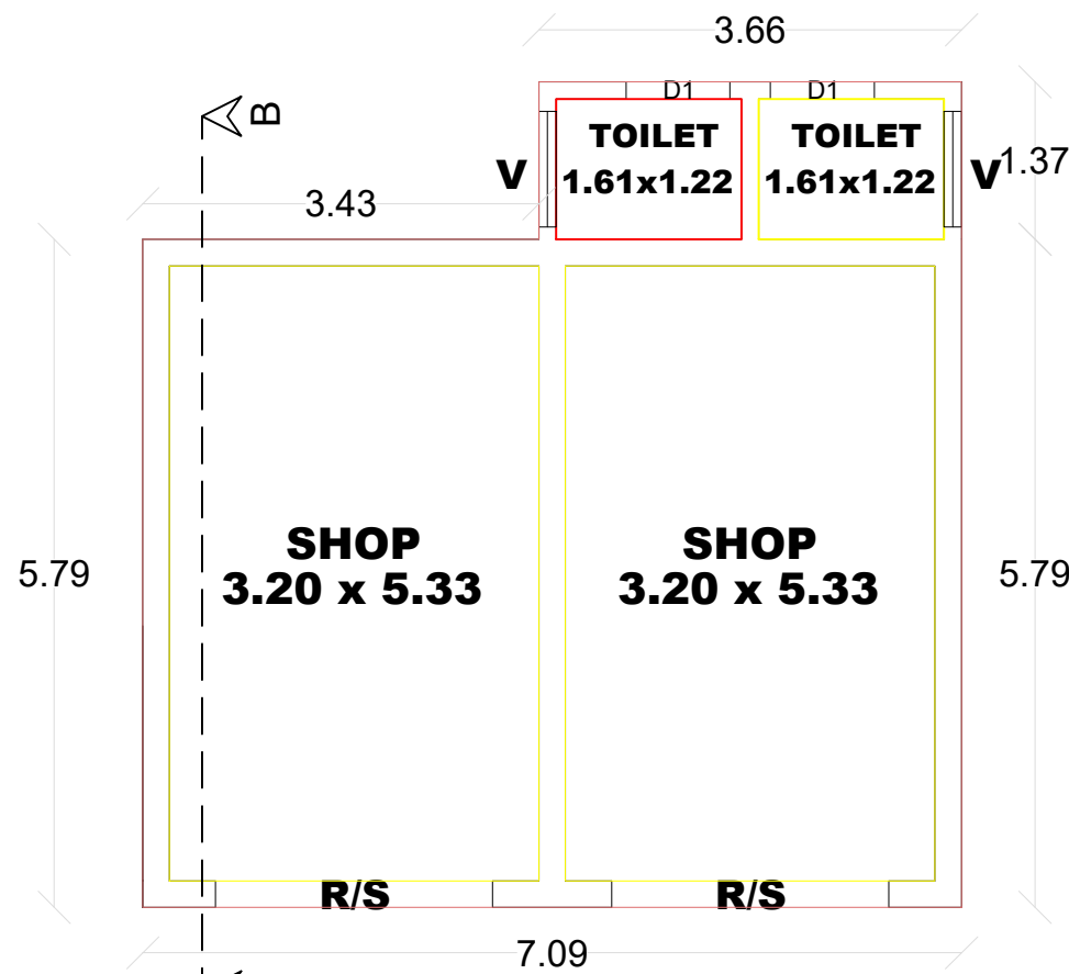
PROPOSED G.F PLAN - 2
