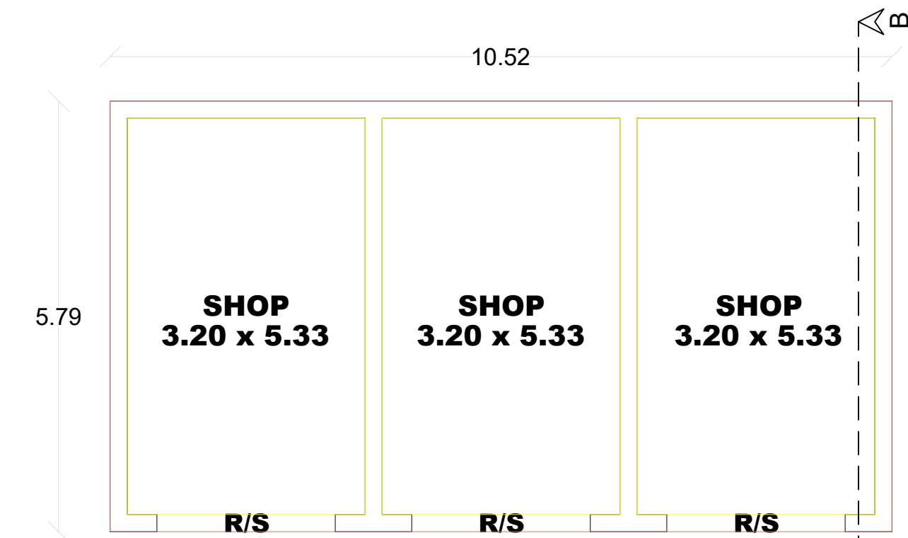
PROPOSED G.F PLAN - 1
