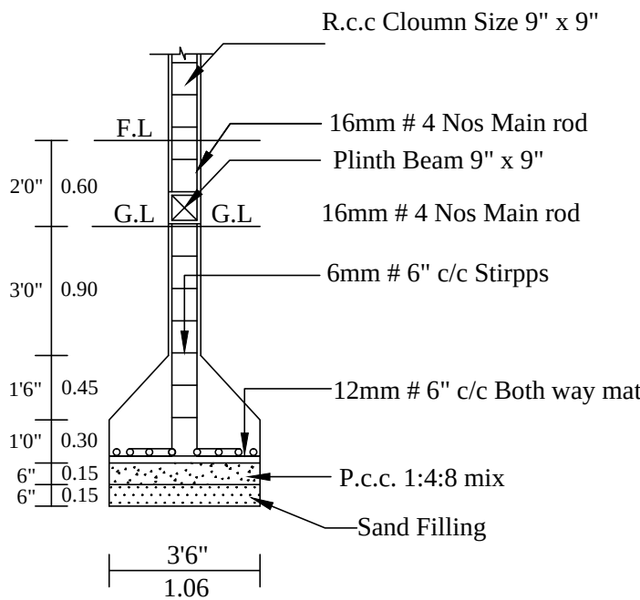
COLUMN DETAILS
