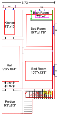
USED FIRST FLOOR PLAN
