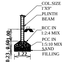
COLUMN DETAILS
