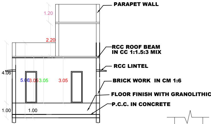
SECTION "A-B"
