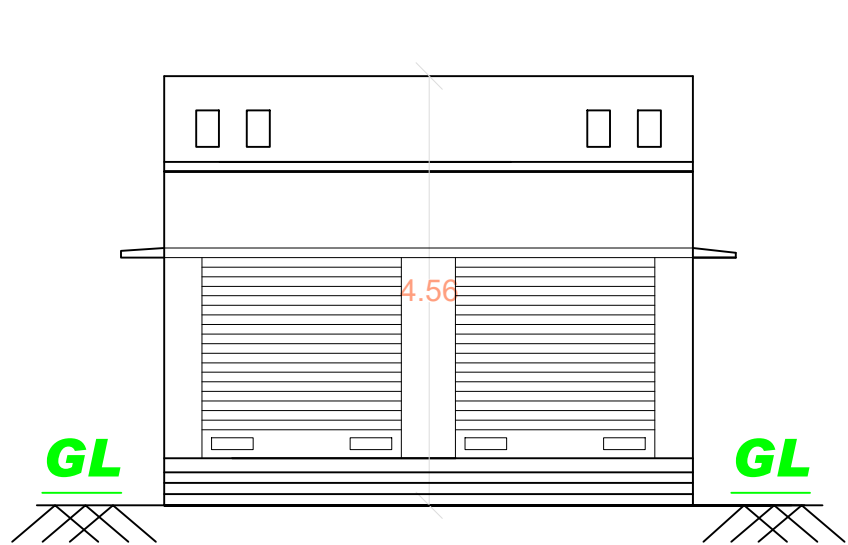
FRONT ELEVATION
