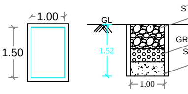
RAIN WATER HARVEST PIT
