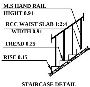
STAIRCASE DETAIL
