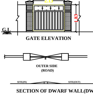
SECTION OF DWARF WALL(DW)
