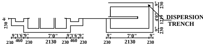
SEPTIC TANK DETAILS.
