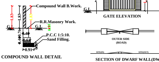
COMPOUND WALL DETAIL
