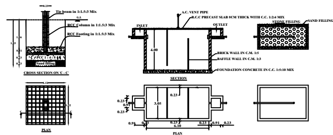
COLOUM FOUNDATION DETAILS - A
