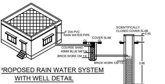
CROSS SECTION OF WELL 4'0" DIA
