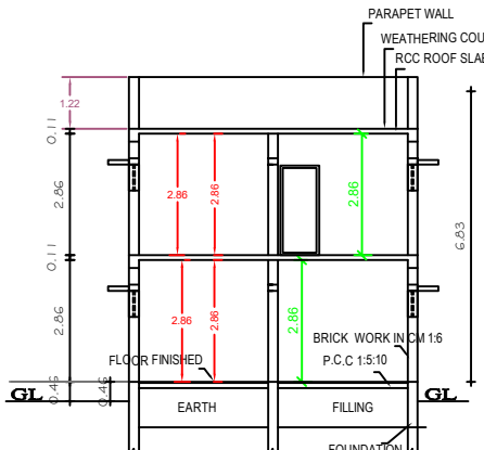
SECTION "A-B"
