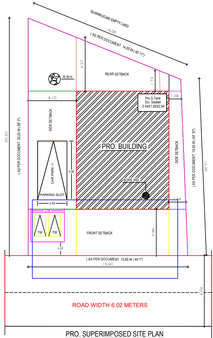
PRO. SUPERIMPOSED SITE PLAN
