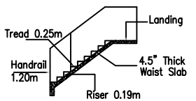
STAIRCASE DETAIL
