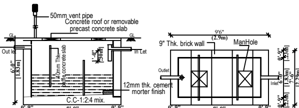
PERCOLATION PIT
