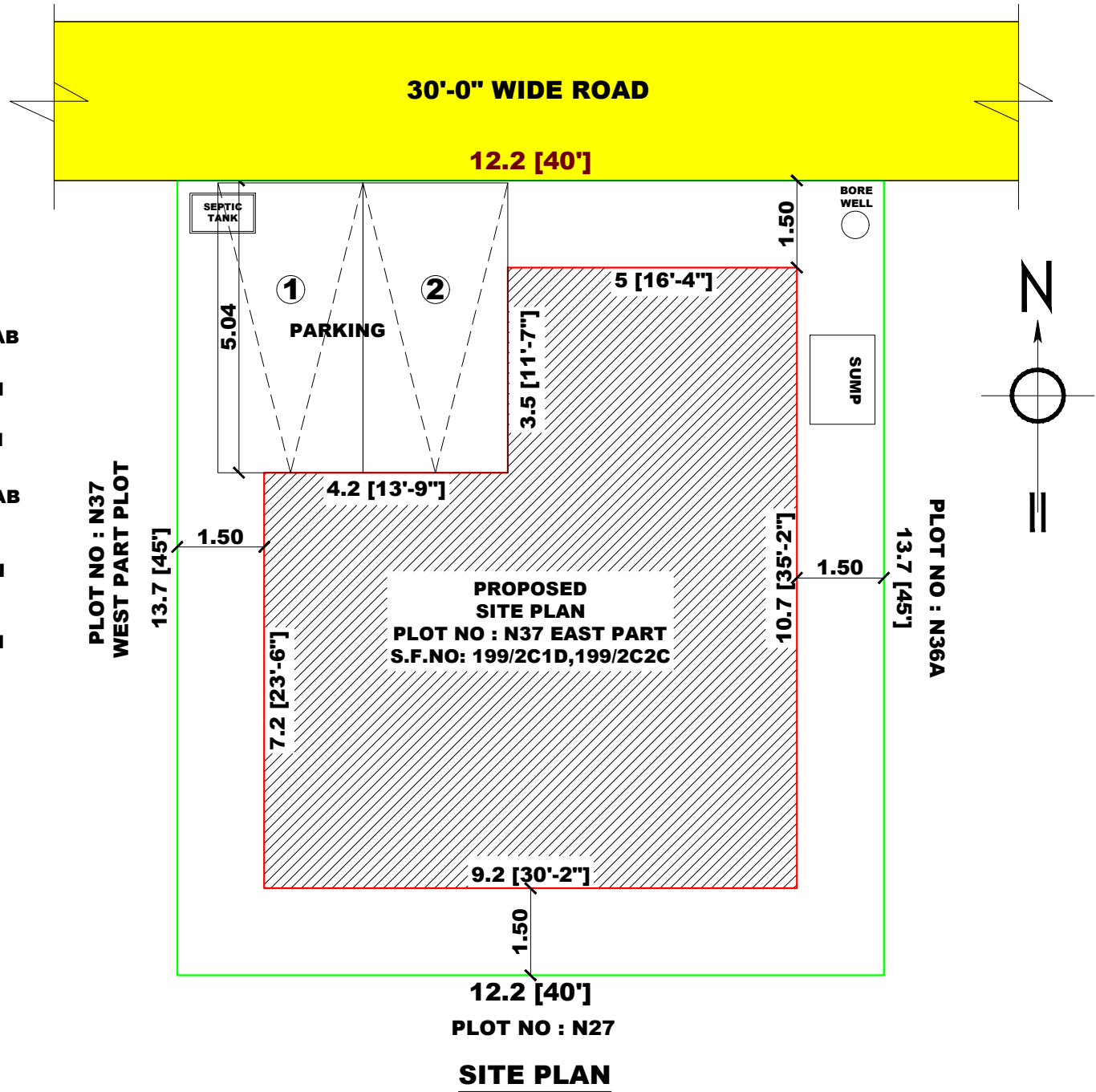
SITE PLAN
