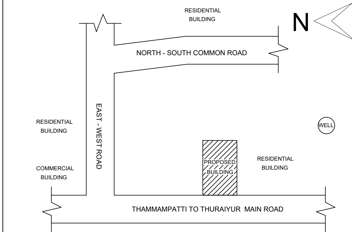
KEY PLAN
