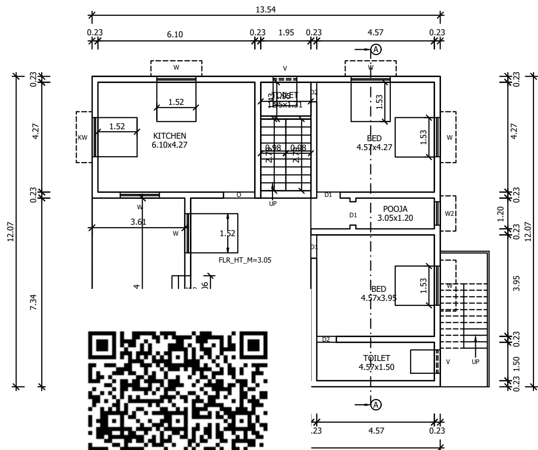
PLAN
