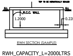
RWH_CAPACITY_L=2000LTRS
