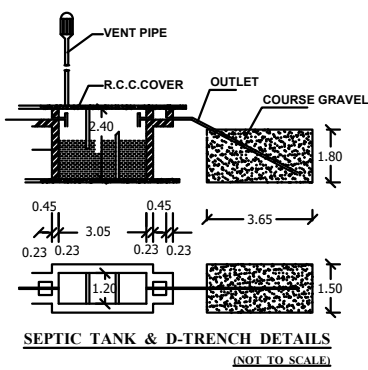
SEPTIC TANK & D-TRENCH DETAILS (NOT TO SCALE)
