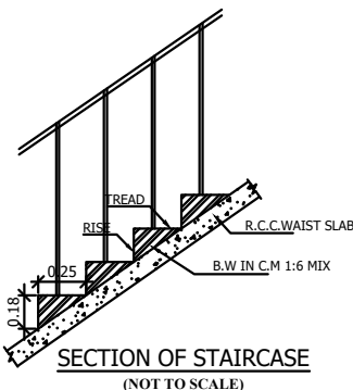
SECTION OF STAIRCASE (NOT TO SCALE)
