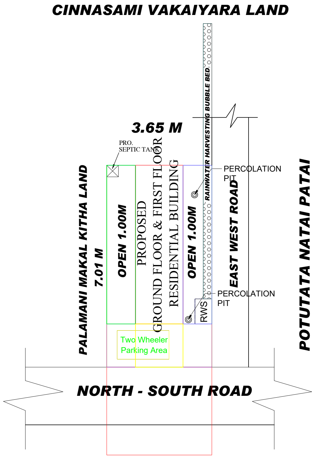
SITE PLAN (SCALE 1:1)
