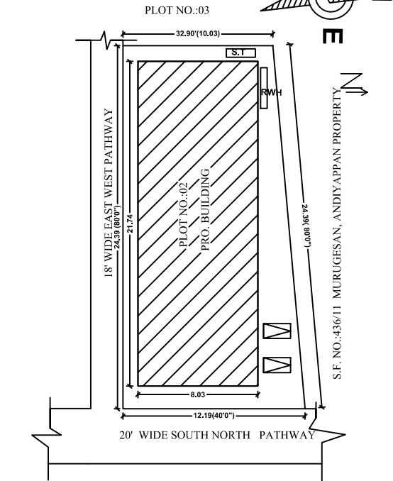
SITE PLAN
