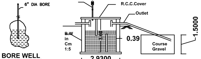
BORE WELL
