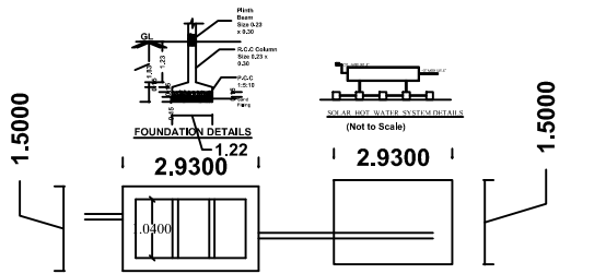
SEPTIC TANK & D-TRENCH DETAILS
