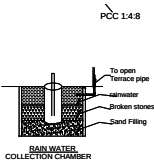
RAIN WATER COLLECTION CHAMBER
