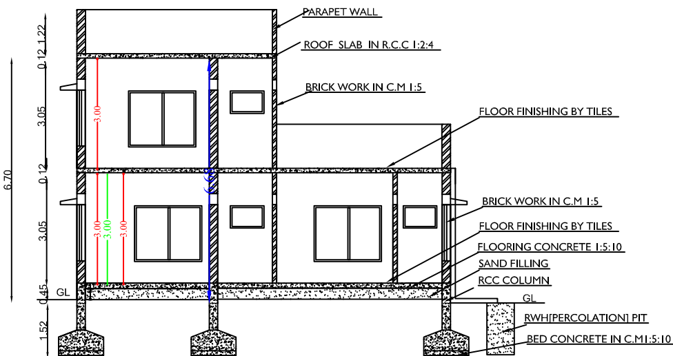
SECTION ON-XY
