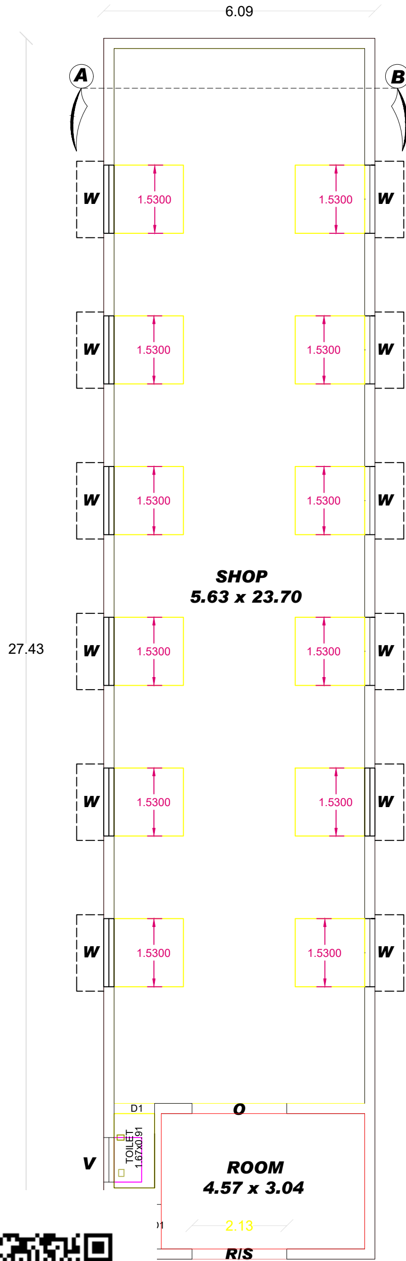
ND FLOOR PLAN
