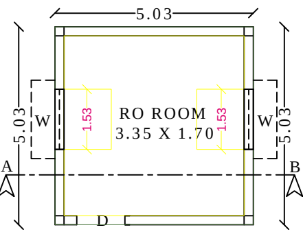
PRO.RO ROOM PLAN
