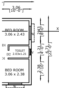
FLOOR PLAN
