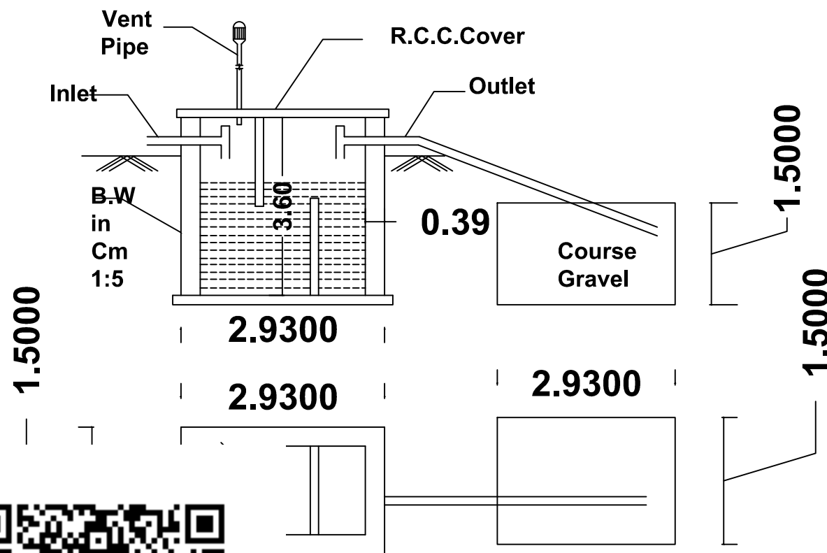
& D-TRENCH DETAILS
