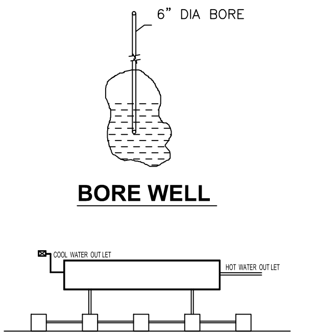
BORE WELL SOLAR HOT WATER SYSTEM DETAILS (Not to Scale)
