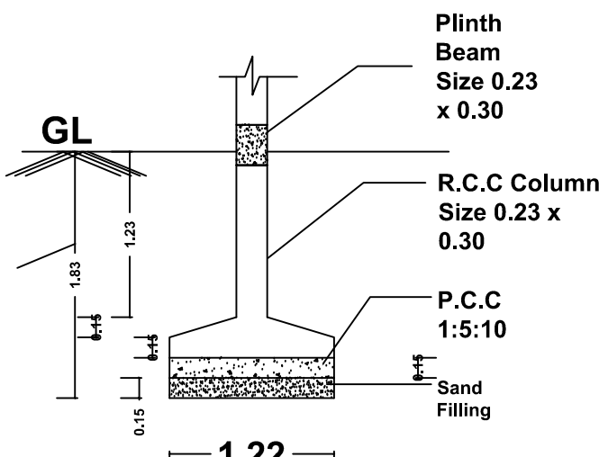
FOUNDATION DETAILS
