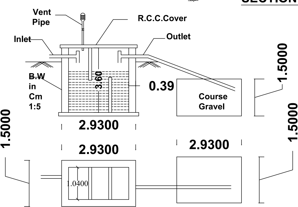
SEPTIC TANK & D-TRENCH DETAILS
