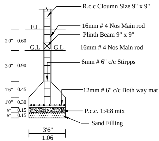
COLUMN DETAILS
