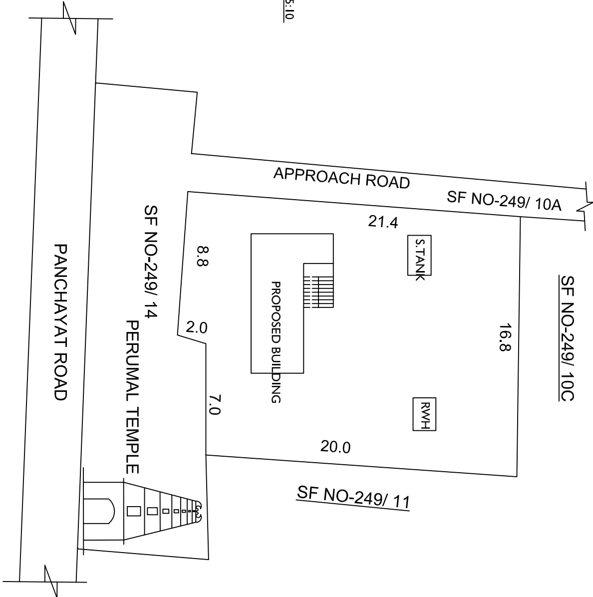
SITE PLAN AS PER FMB
