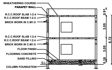
SECTION ON G.G
