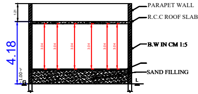
SECTION "AB"
