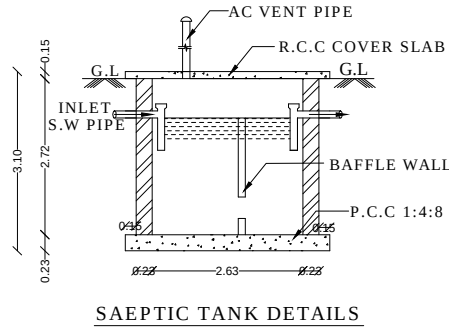
SAEPTIC TANK DETAILS
