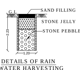
DETAILS OF RAIN WATER HARVESTING
