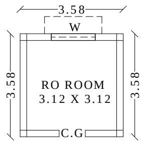
BLOCK -1 PRO.PHASIS RO ROOM
