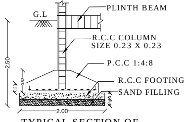
TYPICAL SECTION OF R.C.C COLOUMN FOOTING
