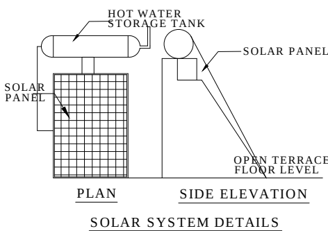
SOLAR SYSTEM DETAILS
