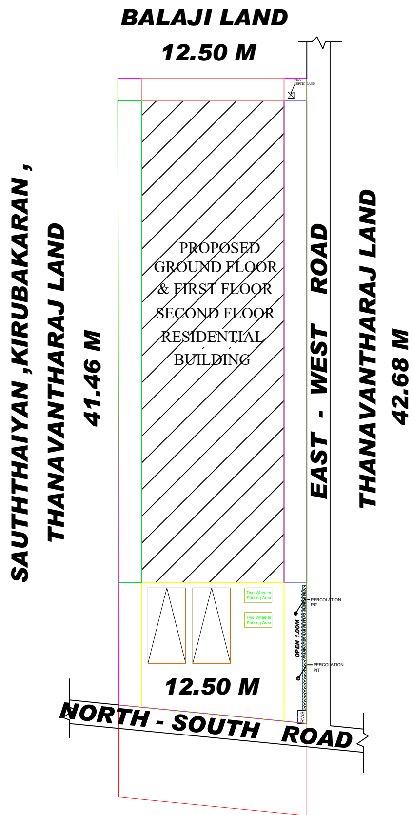
SITE PLAN (SCALE 1:1)
