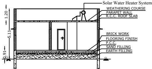
SECTION ON XX
