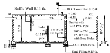
SECTION - SEPTIC TANK & SOAK PIT
