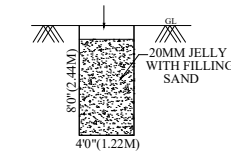
RAIN WATER HARVESTING UNIT
