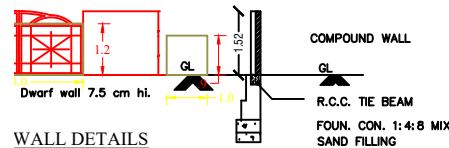
WALL DETAILS
