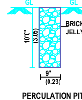
PERCOLATION PIT
