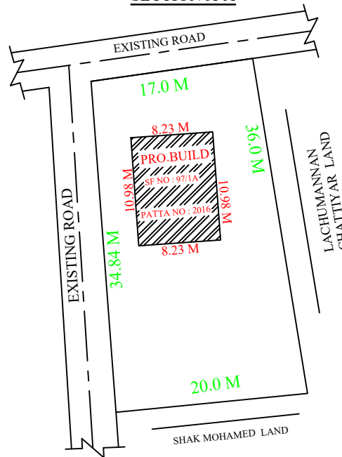
SITE PLAN
