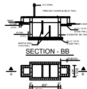
PLAN OF SEPTIC TANK
