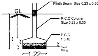
FOUNDATION DETAILS
