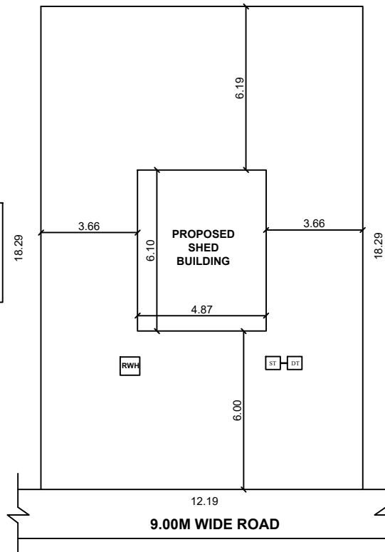
SITE PLAN
