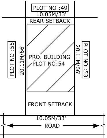
SITE PLAN
