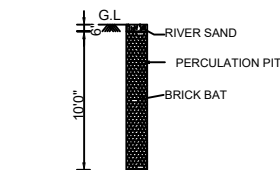
PERCOLATION PIT
