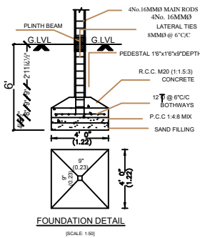
FOUNDATION DETAIL
