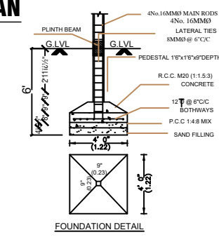
FOUNDATION DETAIL
