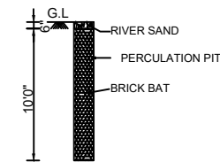
PERCULATION PIT
