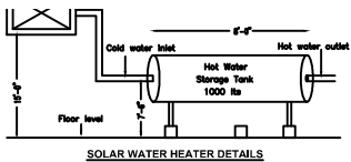
SOLAR WATER HEATER DETAILS
