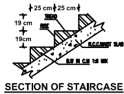
SECTION OF STAIRCASE
