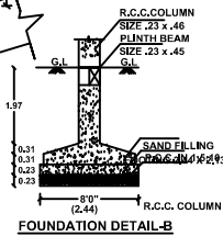
FOUNDATION DETAIL-B
