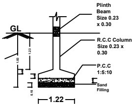
FOUNDATION DETAILS
