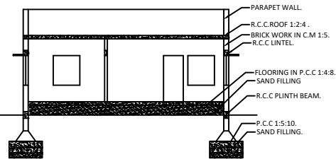
SECTION-RR
