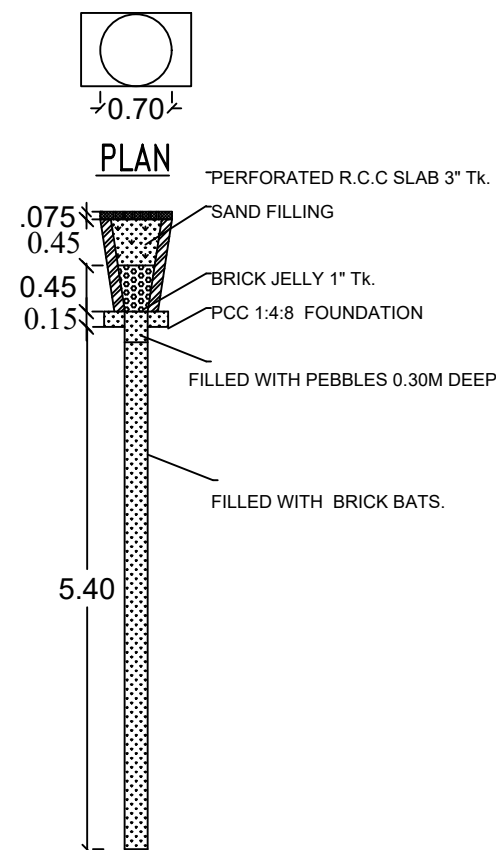
SECTION OF RAIN WATER PERCOLATION PIT
