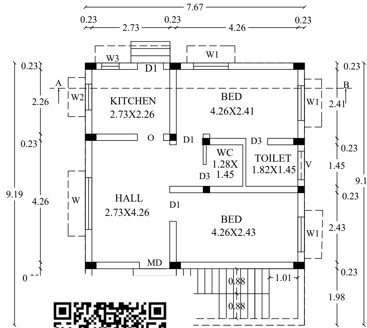
GROUND FLOOR PLAN (NG)
