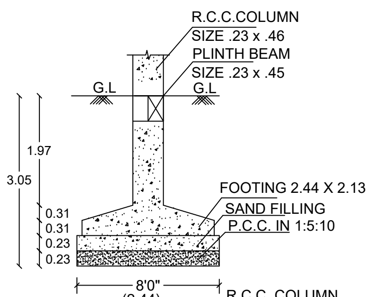
FOUNDATION DETAIL-B
