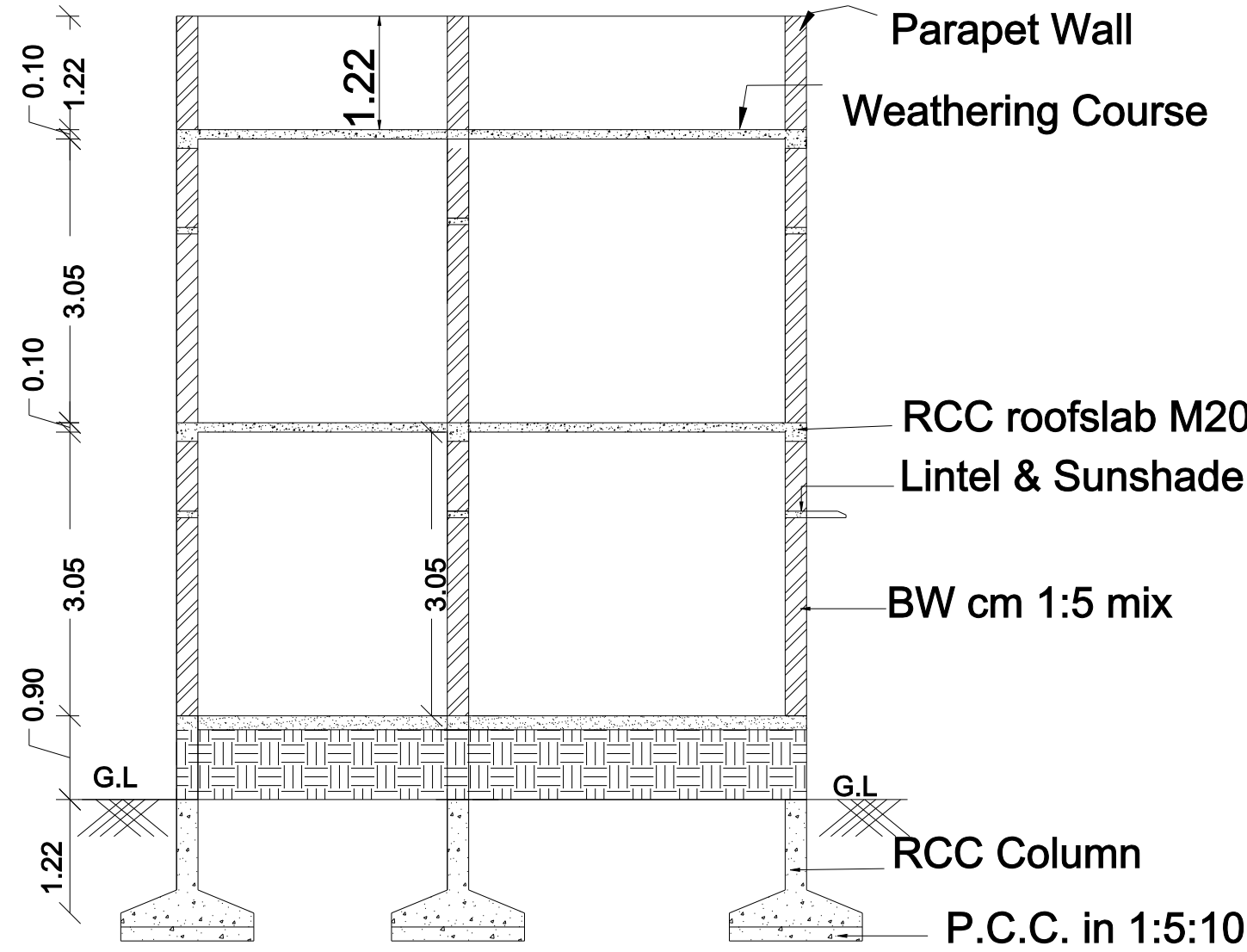
SECTION- BB
