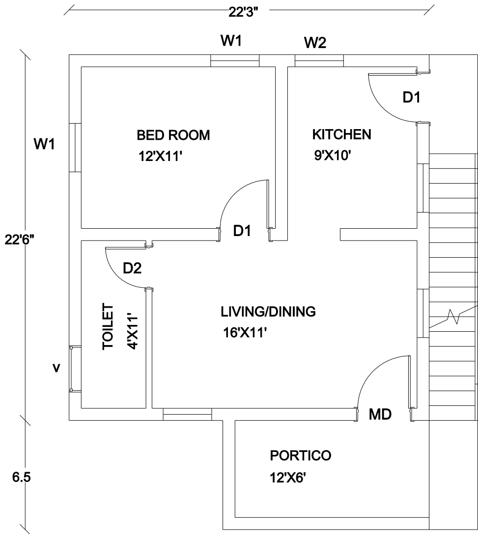
PROPOSED FIRST FLOOR PLAN (RESIDENTIAL)
