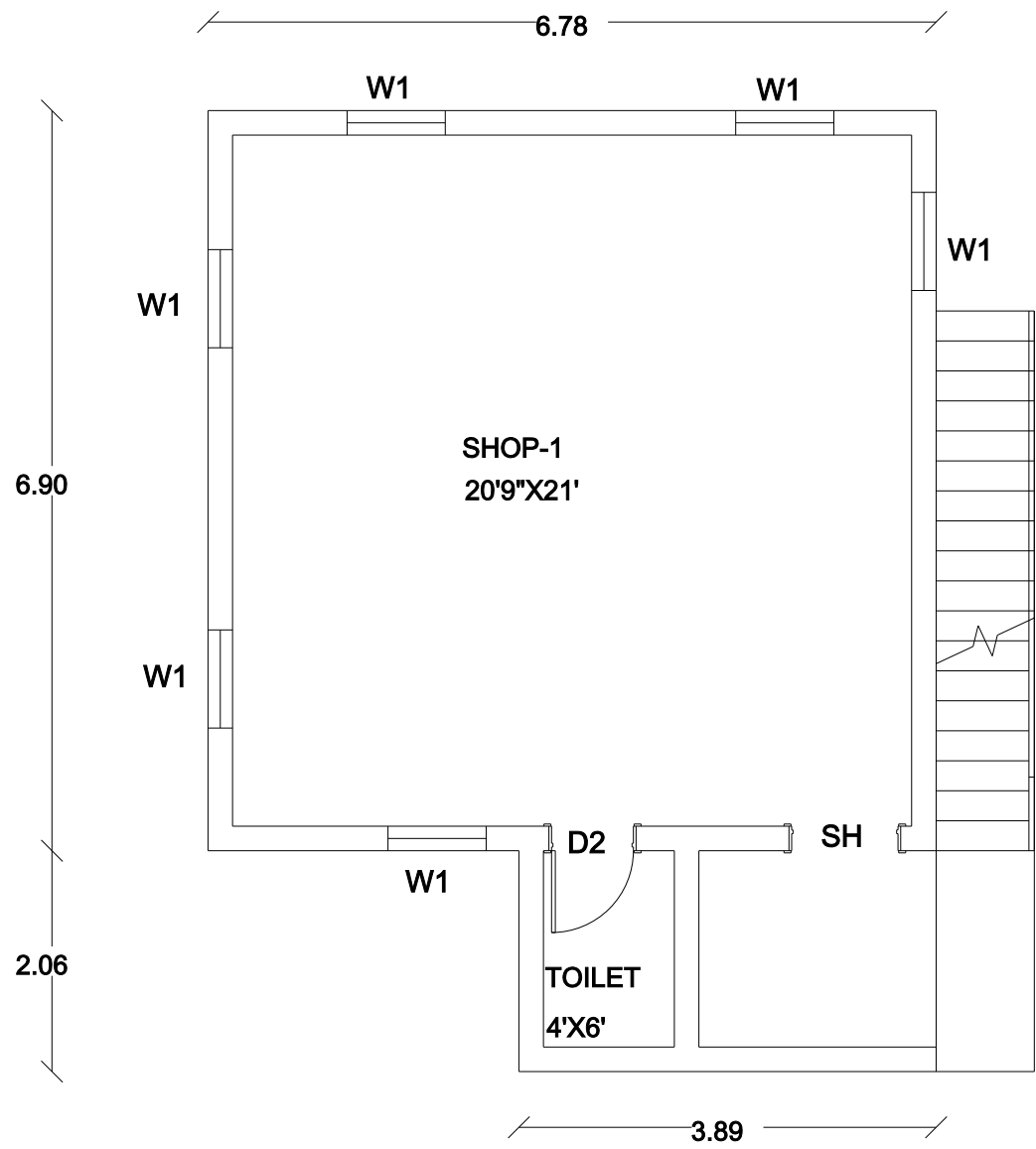
PROPOSED GROUND FLOOR PLAN (COMMERCIAL)
