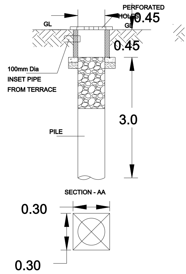
RWHTypicalDetail
