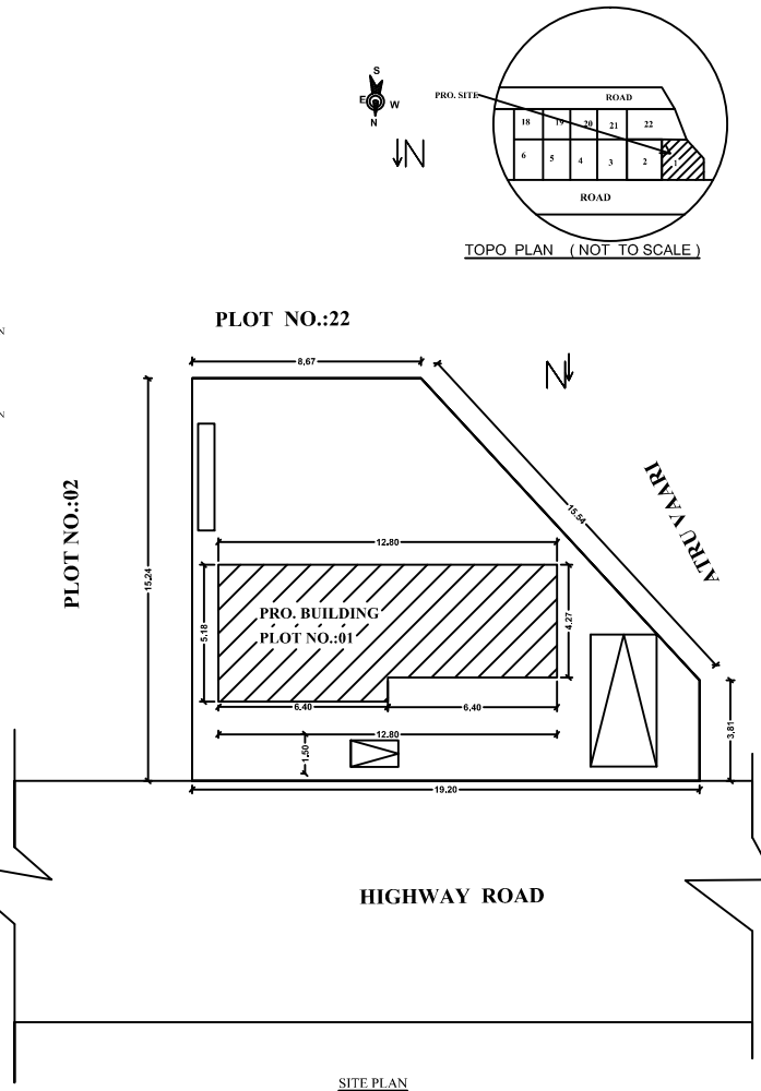
SITE PLAN
