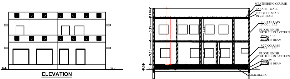
SECTION ON AA
