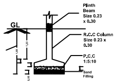
FOUNDATION DETAILS
