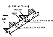
SECTION OF STAIRCASE
