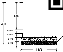
COLUMN FOUNDATION DETAIL (DETAIL - A)
