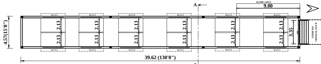
PROPOSED BUILDING PLAN
