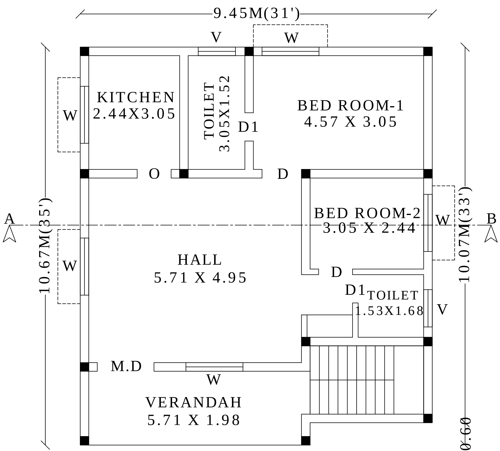
PRO.GROUND FLOOR PLAN (NORTH FACING)
