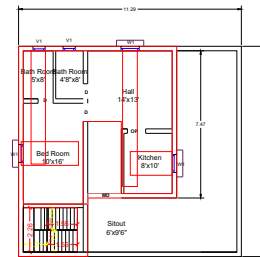
PROPOSED SECOND FLOOR PLAN
