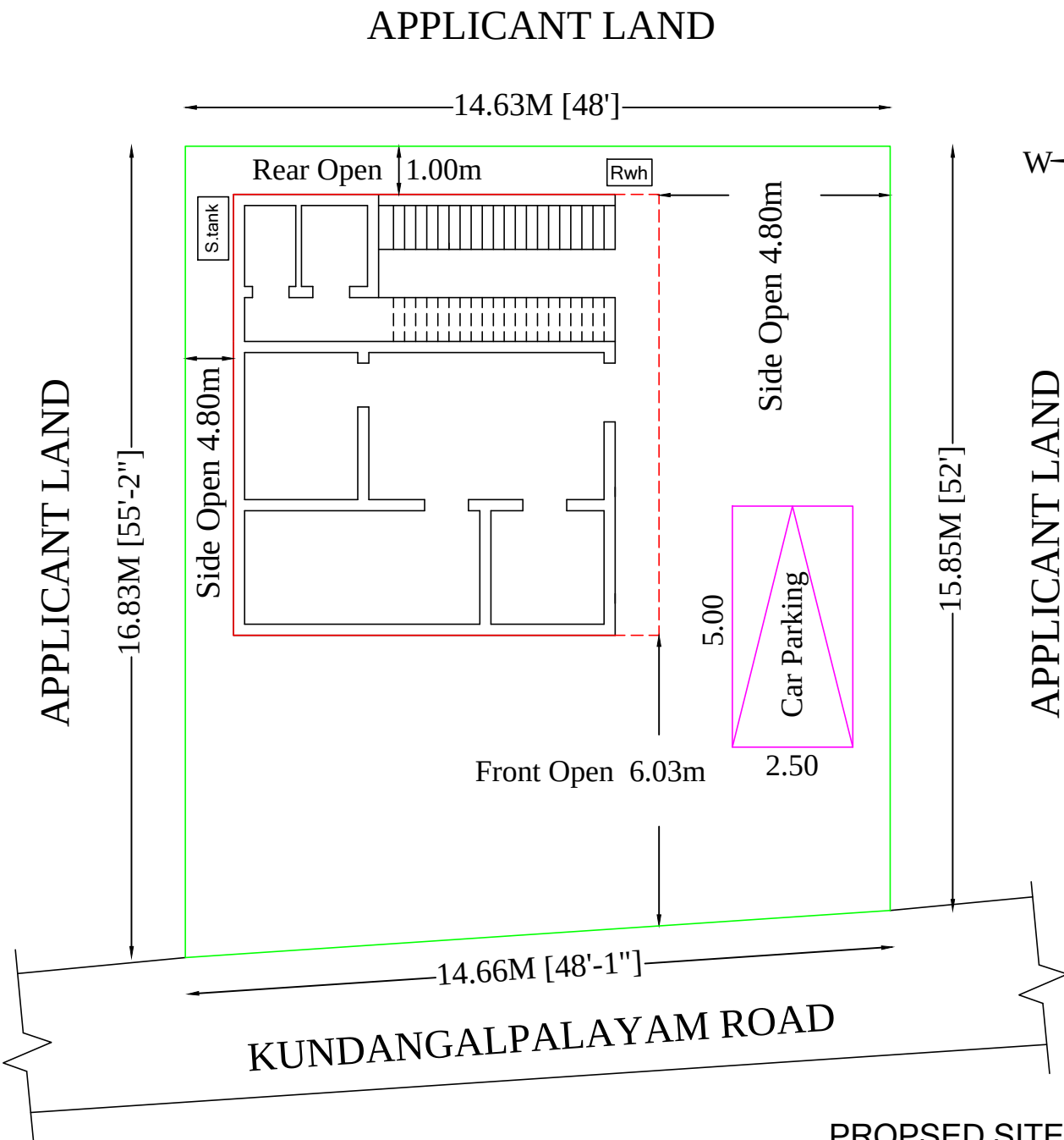
PROPOSED SITE PLAN (SCALE - 1:100)
