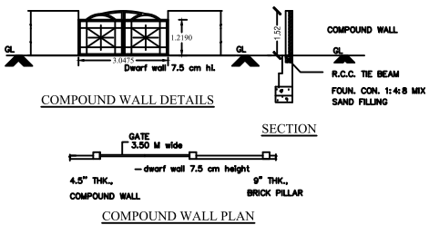
COMPOUND WALL PLAN
