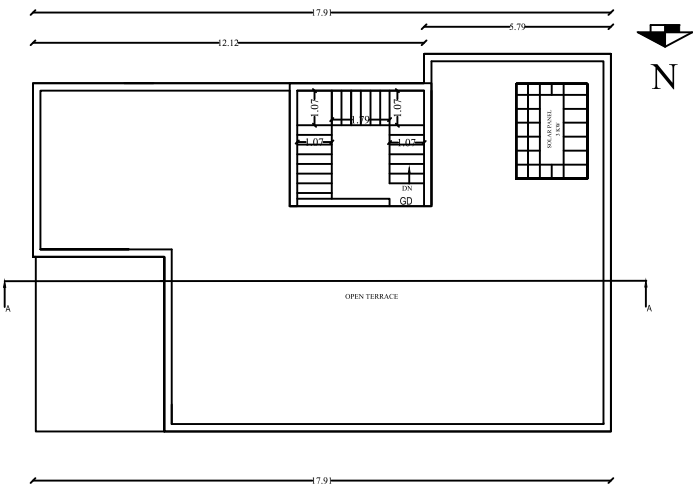
PRO. TERRACE FLOOR PLAN.
